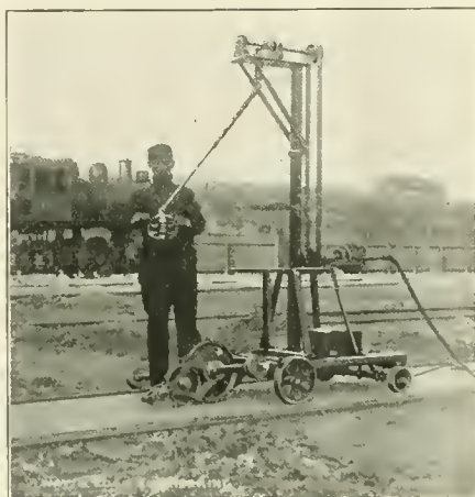
FIG. 1—PORTABLE GRINDER.
